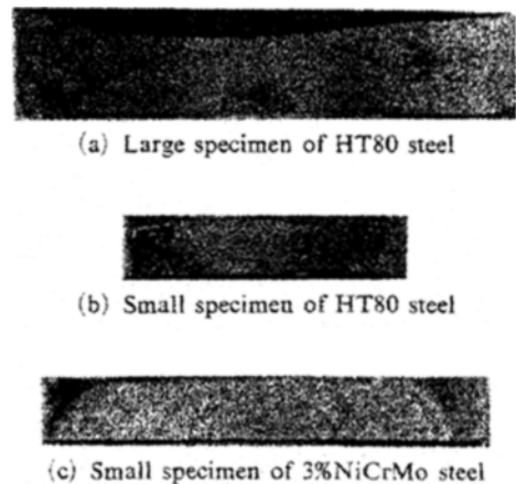
Fig. 2 Photographs of fracture surface obtained from low fatigue load
