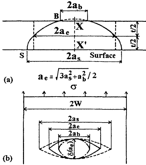
Fig. 3 The crack model used to determine the stress intensity factor after penetration
