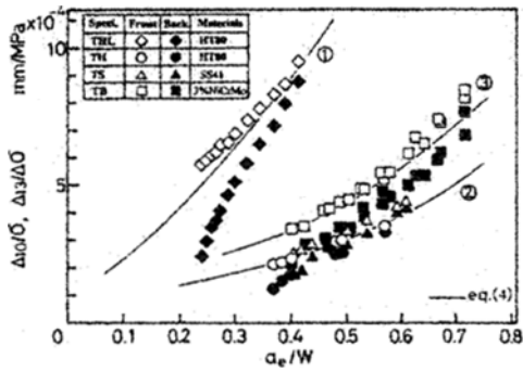
Fig. 4 Comparison of experimental with calculated values at the center of the plate of crack opening displacement
