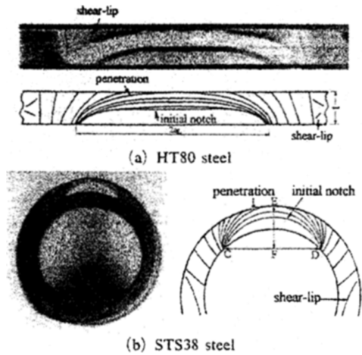
Fig. 5 Photographs of fracture surface obtained from high fatigue load
